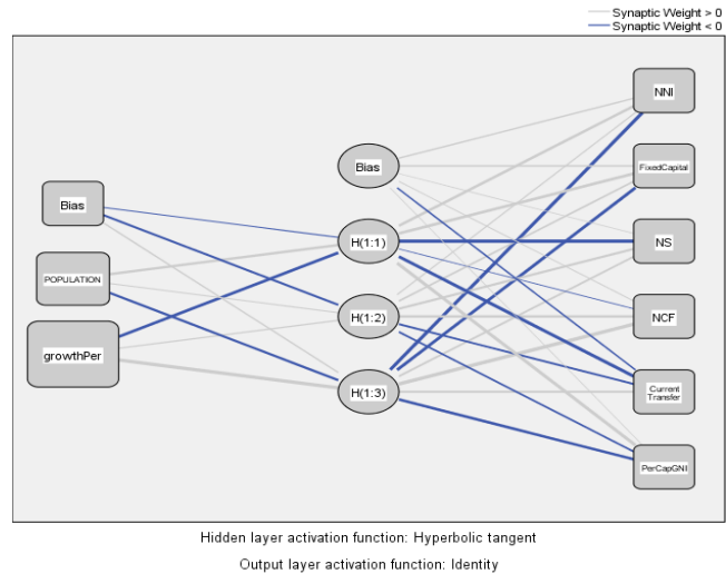
Figure 1: Application of Network Showing Independent Variable Importance
