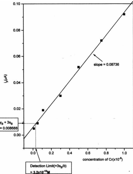
Fig. 9. Determination of detection limit from a linear calibration plot. Data from Fig. 8.
