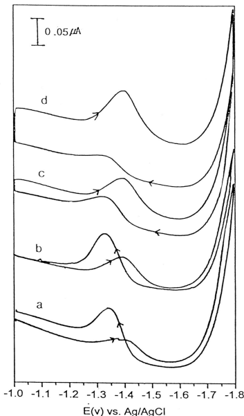
Fig. 7. The effect of scan rate : (a) 10 mV/s, (b) 20 mV/s, (c) 50 mV/s, (d) 100 mV/s on the inverted peak
