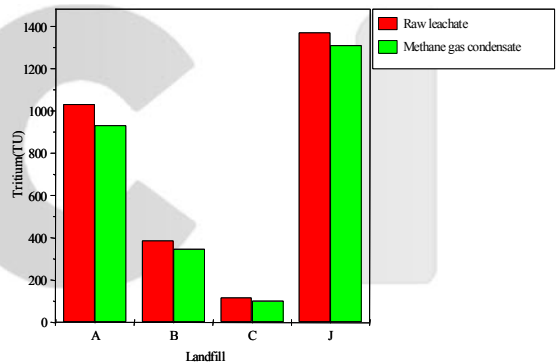
Fig. 3. Tritium level of the raw leachates and condensates of the methane gas for domestic solid waste landfills.
