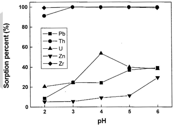
Fig. 2. Effect of pH on sorption of metal ions with XAD-16-CTA chelating resin. Resin weight: 15 mg, Conc. of metal ion: each 10 µg/mL/15 mL, Shaking time: 24 hrs.
