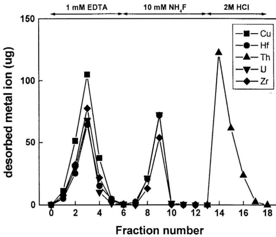
Fig. 10. Separation of Th(IV) from mixed metal ions with XAD-16-CTA chelating resin. Resin weight : 100 mg, Conc. of metal ion : each 10 μg/mL, Sorption flow rate : 0.2 mL/min, Desorption flow rate : 0.1 mL/min.
