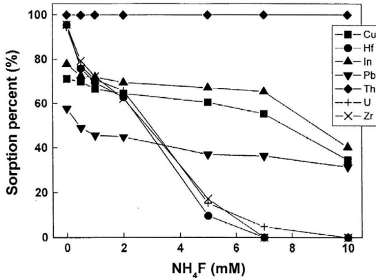
Fig. 8. Effect of NH 4 F on sorption of metal ions with XAD-16-CTA chelating resin. Resin weight : 15 mg, Conc. of metal ion : each 10 µg/mL/15 mL, Matrix : pH 4, 0.01M HAc-NH 4 Ac buffer solution, Shaking time : 24 hrs.
