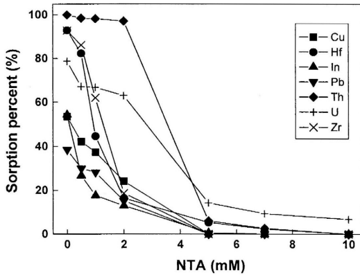
Fig. 7. Effect of NTA on sorption of metal ions with XAD-16-CTA chelating resin. Resin weight : 15 mg, Conc. of metal ion : each 10 µg/mL/15 mL, Matrix : pH 4, 0.01 M HAc-NH 4 Ac buffer solution, Shaking time : 24 hrs.
