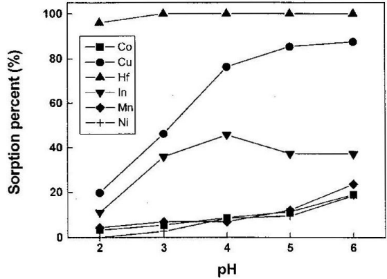
Fig. 1. Effect of pH on sorption of metal ions with XAD-16-CTA chelating resin. Resin weight: 15 mg, Conc. of metal ions: each 10 µg/mL/15 mL, Shaking time: 24 hrs.
