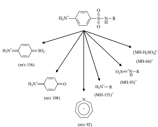
Fig. 4. Proposed MS/MS fragmentation pathways for protonated sulfonamides. 7
