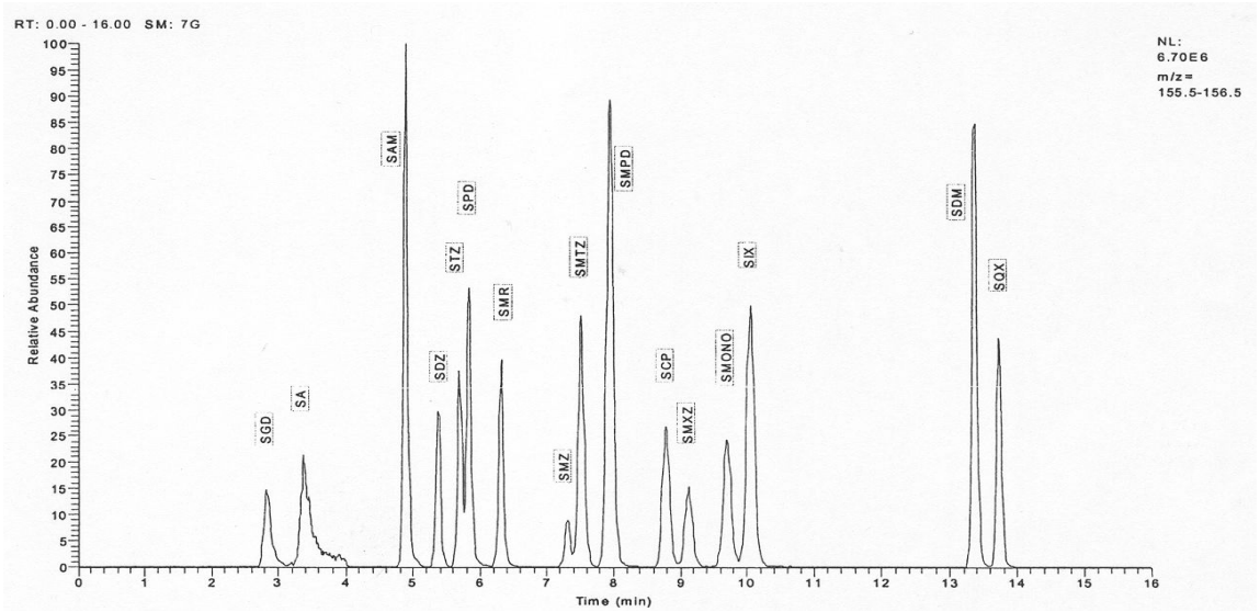
Fig. 9. Example of chromatogram from time-scheduled MS/MS, showing the ion chromatogram for m/z 156 common to various sulfonamides. 30
