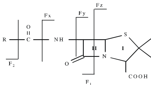
Fig. 5. Proposed MS/MS fragmentation pathways for \beta -lactam antibiotics; [F_x+H]^+ = 217 , [F_x-COOH]^+ = 226 , [F_y+H]^+ = 202 , [F_y+H-CO]^+ = 174 , [F_z+H]^+ = 160 , [F_z-COOH]^+ = 114 ; [F_1+H]^+ , [F_2+H]^+. 2
