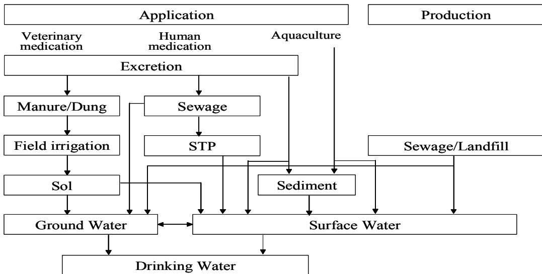
Fig. 10. Possible pathways of antibiotics into the environmental. 31
