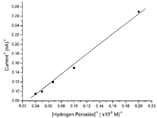
Fig. 4. Lineweaver-Burk plot from the data in Fig. 3.
