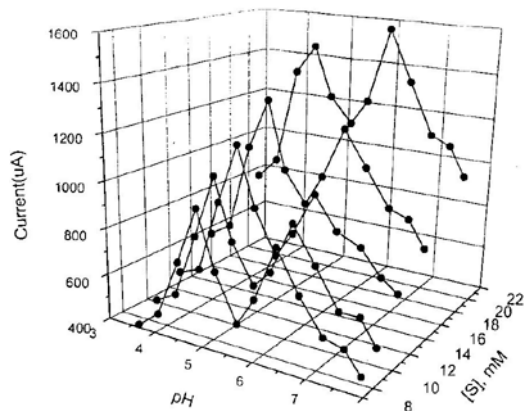
Fig. 6. pH-dependent current responses at the five different concentrations of substrate.
