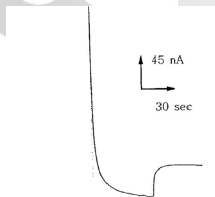
Fig. 2. Typical response curve of the biosensor. 0.1 M H_2O_2 , 100 uL was added to 10 mL electrolyte solution (pH 8.47) at -100 mV (vs. Ag/AgCl). The tissue composition of the electrode used was 5%.
