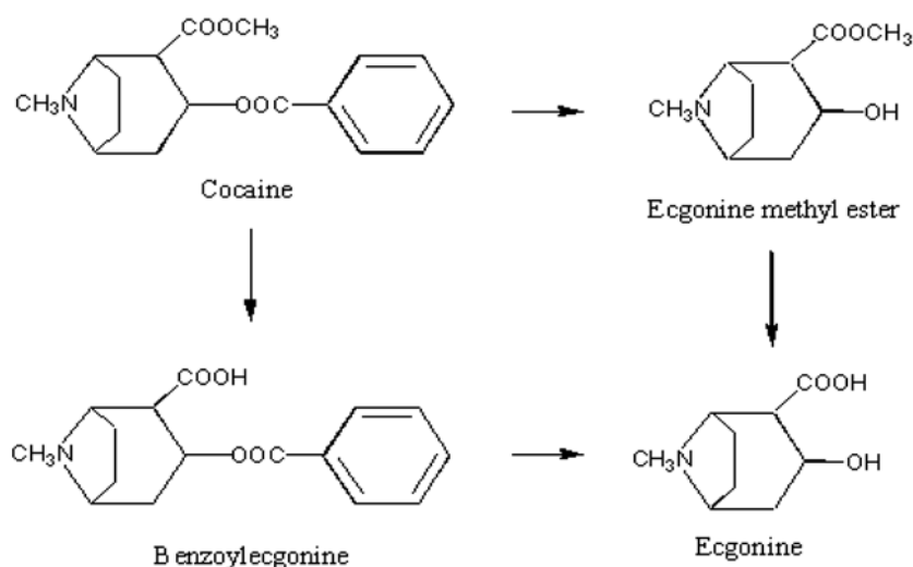
Fig. 3. Metabolic pathway of cocaine. It's major metabolites are benzoylecgonine (BE) and ecgonine methylester (EME).
