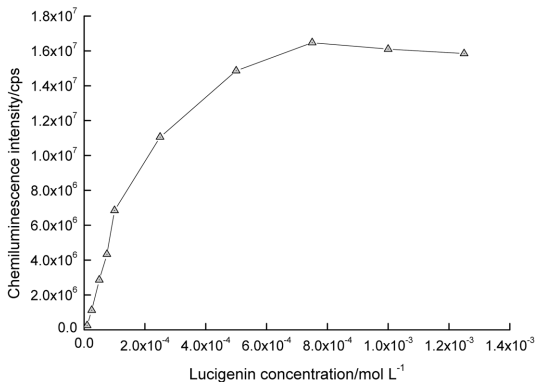
Fig. 5. Effect of concentration of lucigenin on the chemiluminescence intensity of lucigenin-H 2 O 2 in the presence of vitamin P 1 . Conditions: pH, 11.4; vitamin P 1 , 1.0×10 -3 mol/L; H 2 O 2 , 0.5 mol/L; λ em =473 nm.
