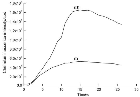
Fig. 6. CL kinetic curves of system; (I): lucigenin-H 2 O 2 in the absence of vitamin P 1 ; and system (II): lucigenin-H 2 O 2 in the presence of vitamin P 1 . Conditions: lucigenin, 7.5×10 -4 mol/L; vitamin P 1 , 1.0×10 -3 mol/L; H 2 O 2 , 0.5 mol/L; pH, 11.4; λ em =473 nm.
