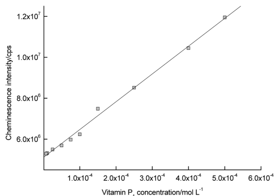
Fig. 7. Calibration curve for vitamin P 1 . Conditions: lucigenin, 7.5×10 -4 mol/L; pH, 11.4; H 2 O 2 , 0.5 mol/L; λ em =473 nm.
