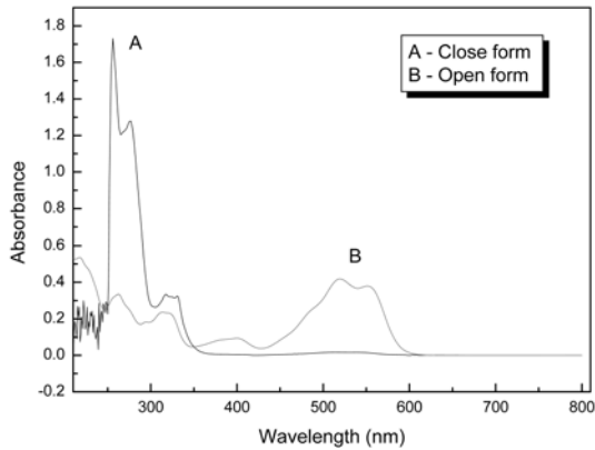
Fig. 1. The UV-Vis spectra of Red-DCF in methanol solution.
