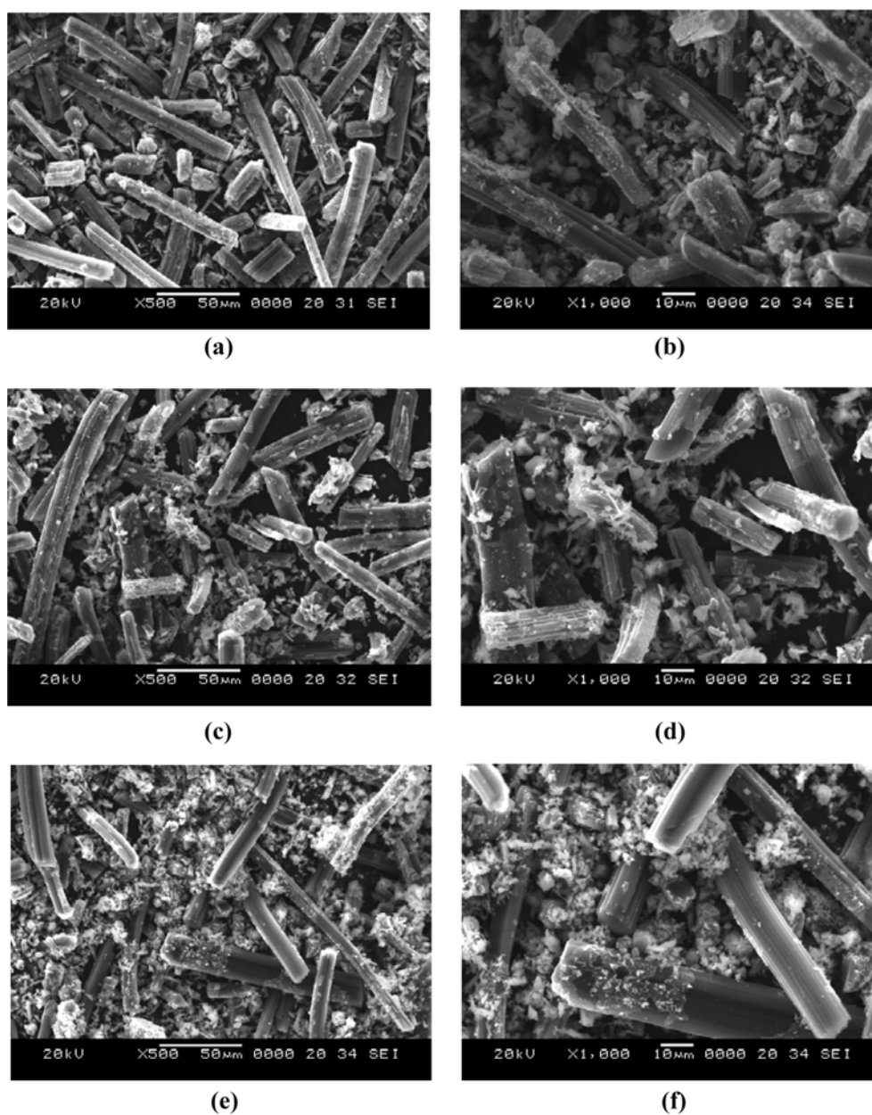
Fig. 1. SEM images of Fe-ACF/TiO 2 composites: FT1: (a) ×500, (b) ×1000; FT2, (c) ×500, (d) ×1000 and FT3 (e) ×500, (f) ×1000.
