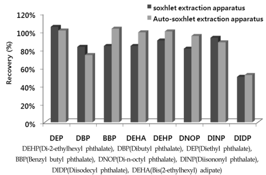
Fig. 1. Recoveries of phthalate according to extraction apparatus types(n=5).
