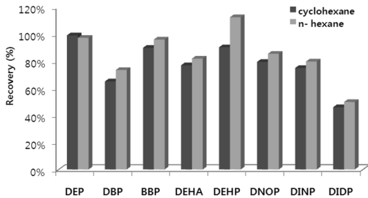
Fig. 4. Efficiency of liquid/liquid extraction according to solvent(n=3).
