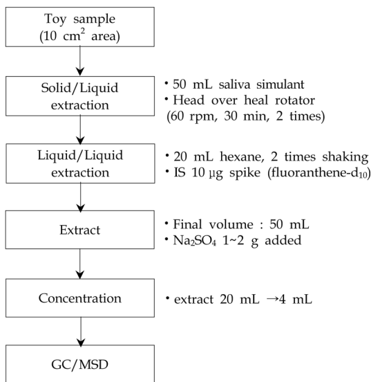
Fig. 5. Flowchart of analytical method for phthalate migration rate(mouthing) in plastic toys.
