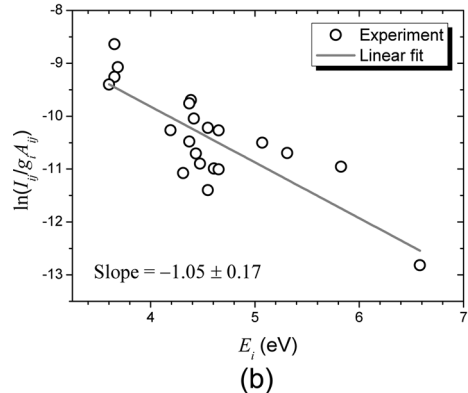
Fig. 4. Boltzmann plots obtained from LIBS spectra of a steel sample in (a) air and (b) He gas flow.
