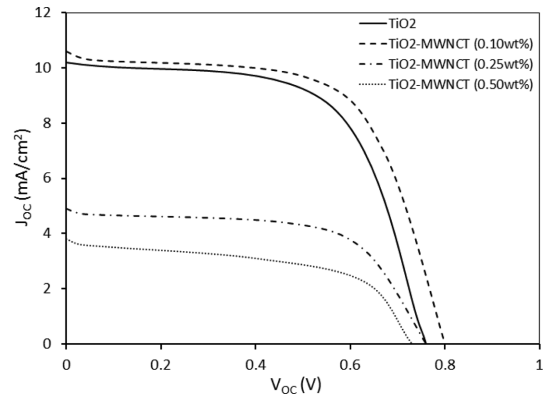
Fig. 5. J-V curves of DSSCs based on TiO 2 -MWNT electrodes.
