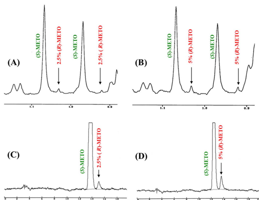
Fig. 6. Typical ^1\text{H-NMR} spectra (A), (B) and chromatograms (C), (D) of synthesized METO mixtures with 2.5 and 5.0% isomeric impurity. HPLC condition: Phenomenex Prodigy silica column (5 \mu\text{m} , 250 \times 4.6 mm), mobile phase: n-hexane/dichloromethane/methanol = 200/200/1, flow rate: 1.0 mL/min, UV detection at 276 nm, injection volume: 5 \mu\text{L} .
