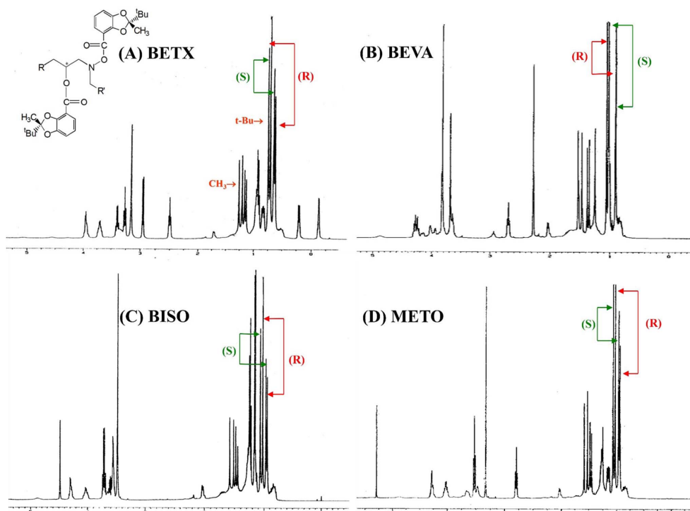
Fig. 4. ^1\text{H-NMR} spectra of ( rac )- \beta -blockers.
