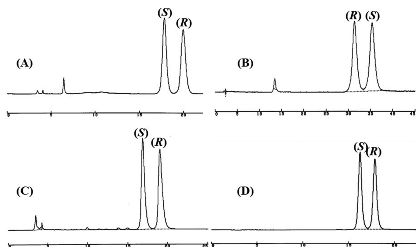
Fig. 5. Chromatograms of diastereomeric derivatives obtained from racemic \beta -blockers after derivatization with ( S )-TBMB-COCl. (A) BETX, (B) BEVA, (C) BISO, (D) METO. Conditions are presented in Table 2.
