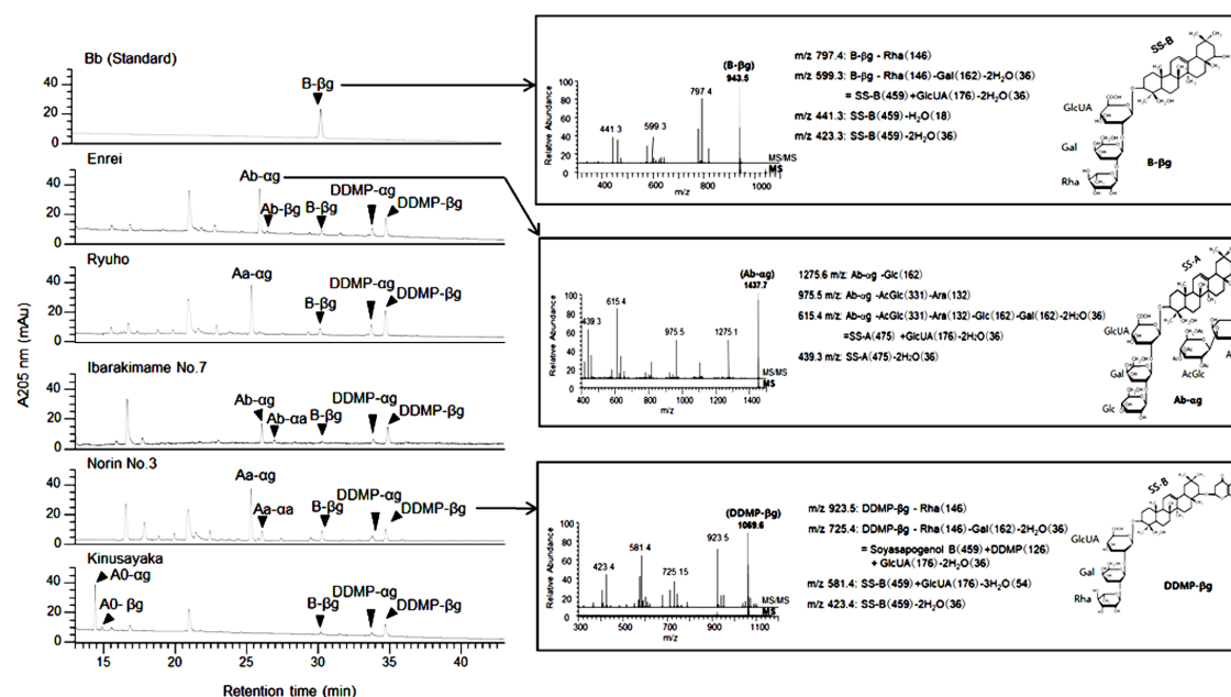
Fig. 2. Comparison of soyasaponins between standard (B- \beta g) and three samples in the hydrolysis extracts. Left: UV results, Right: soyasaponin chemical structures elucidated by MS/MS fragmentation.
