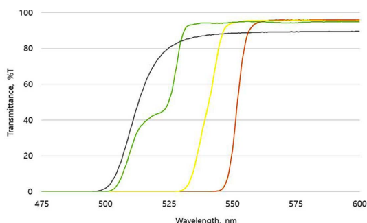
Fig. 4. Comparison of transmittance spectra of ILPF550 filter tilted at various angles and OG515 filter (Orange line: ILPF550 tilted to 0^\circ , Yellow line: ILPF550 tilted to 22.5^\circ , Green line: ILPF550 tilted to 45^\circ , Gray line: OG515).
