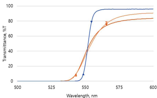
Fig. 1. Transmittance spectrum of absorption filters (OG550, CUSP) and interference filter (ILPF550), (Blue line: ILPF550, Pale orange line: CUSP, Orange line: OG550, ▲: 10 % transmittance coordinates, ▼: 80 % transmittance coordinates).
