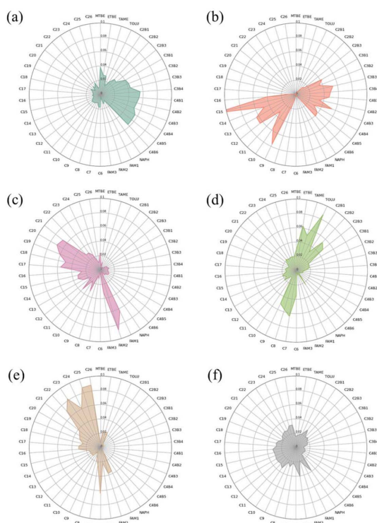
Fig. 5. Mean base peak intensity ratio of each marker component from GC-MS data of fire residues, which were concluded as (a) gasoline, (b) kerosene, (c) diesel, (d) organic solvents, (e) candles, and (f) no fire accelerants were involved.
