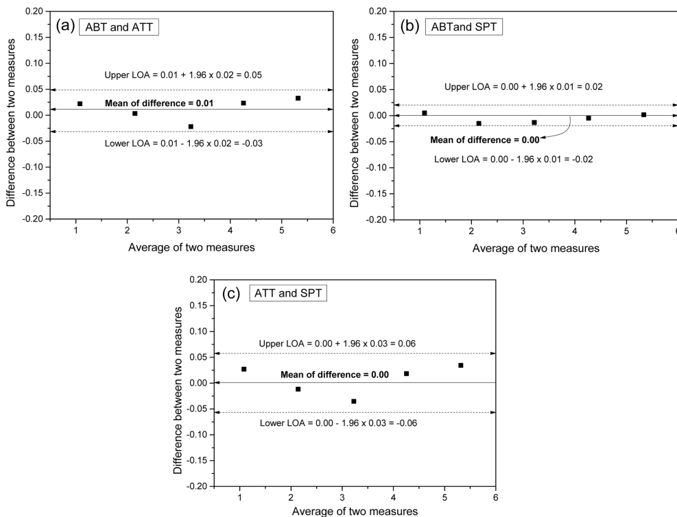
Fig. 4. Bland-Altman plots for analyzing the agreement (a) between ABT and ATT, (b) between ABT and SPT, and (c) between ATT and SPT.
