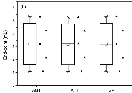
Fig. 3. Q-Q plots (a) and ANOVA bar charts (b) of measured data by three titration equipment.
