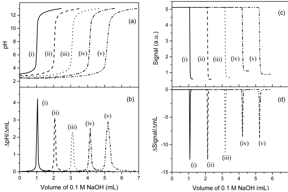
Fig. 1. Titration curves of 0.1 M HCl with 0.1 M NaOH when the volume of 0.1 M HCl is (i) 1 mL, (ii) 2 mL, (iii) 3 mL, (iv) 4 mL, and (v) 5 mL. (a)-(b) and (c)-(d) are obtained by ATT and SPT, respectively.
