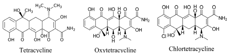
Fig. 1. Chemical structure of tetracyclines (TCs).
