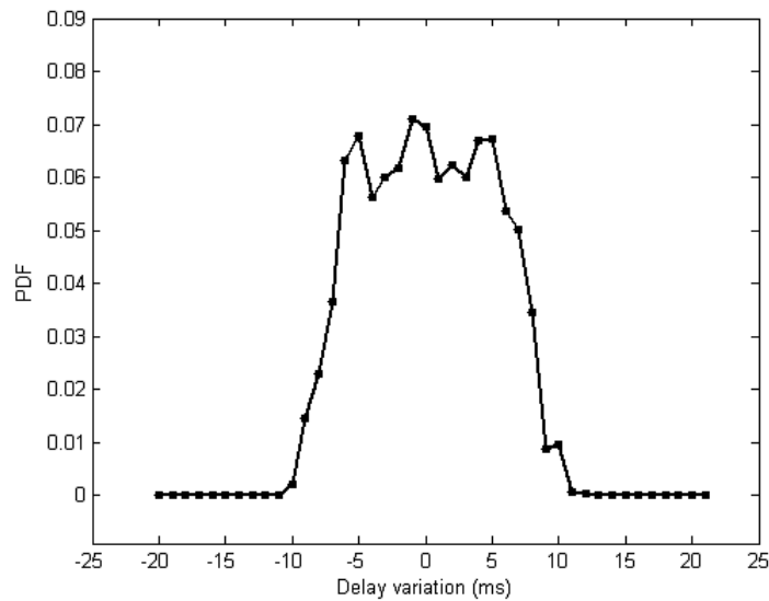
Fig. 3. PDF of measured network delay
