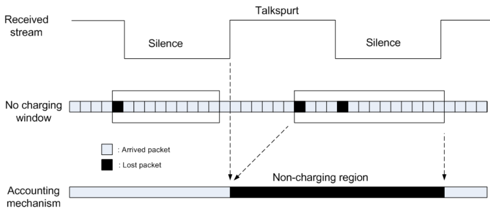
Fig. 8. VoIP charging mechanism
