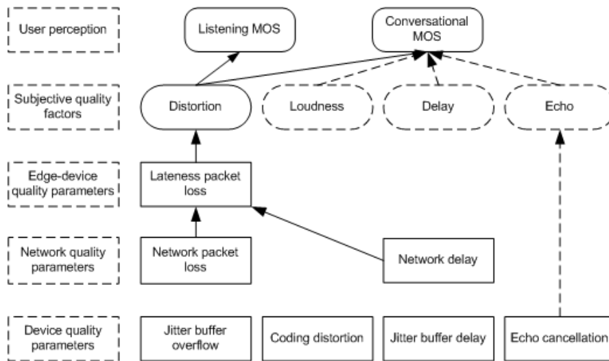
Fig. 1. Parameters that determine the VoIP quality
