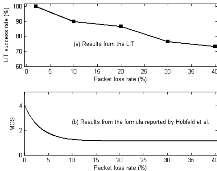
Fig. 7. Comparisons of (a) LIT success rate with (b) estimated MOS value
