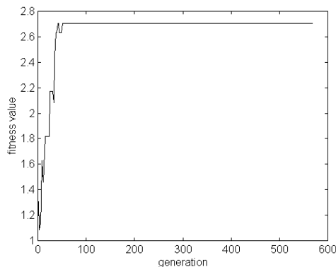
Fig. 5. Fitness value of the processor P_6
