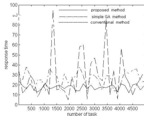
Fig. 4. Result of response time
