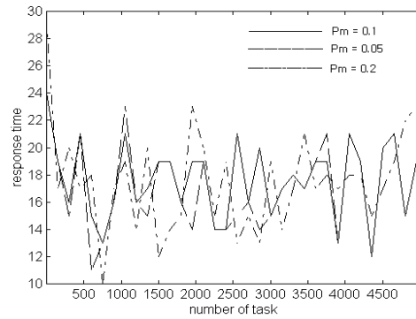
Fig. 7. Result depending on the changes of P_m
