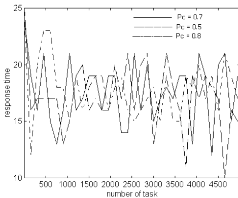
Fig. 6. Result depending on the changes of P_c
