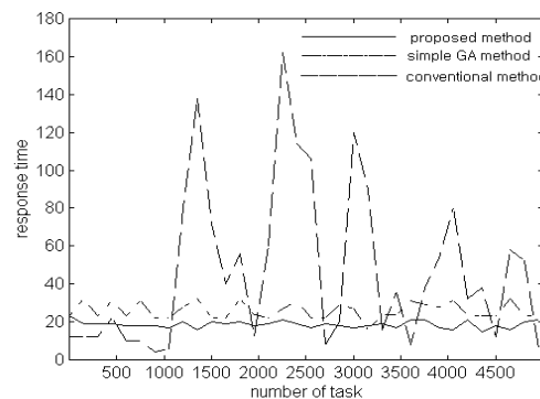
Fig. 8. Response time when system load is 80%
