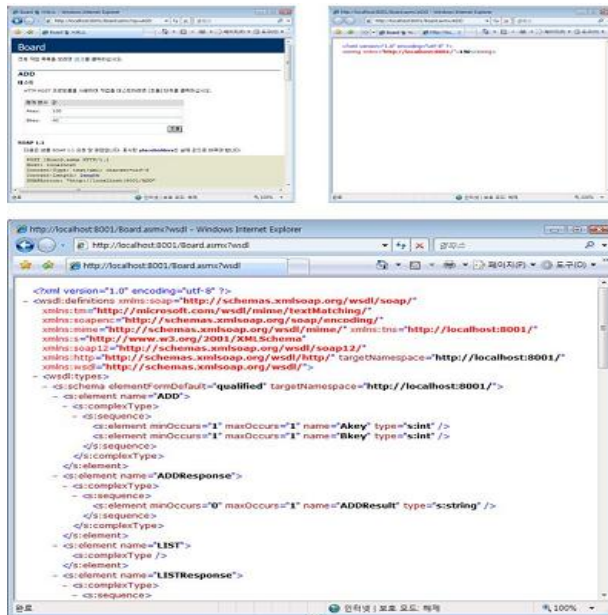
Fig. 6. An example of a SOAP call
