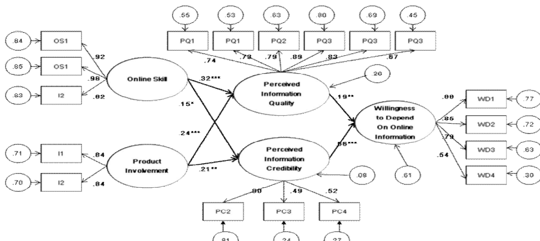
Fig. 2. Standardized structural equation model with parameter estimates
