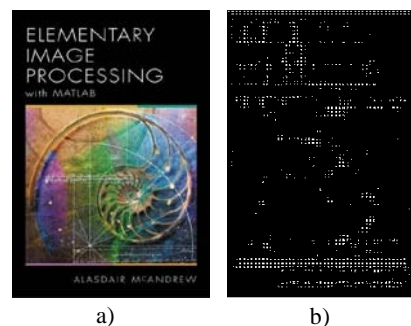
Fig. 3. Process of detecting lines of text. a) Input image; b) Regions that are text candidates;
