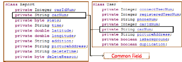
Fig. 6. A class structure
