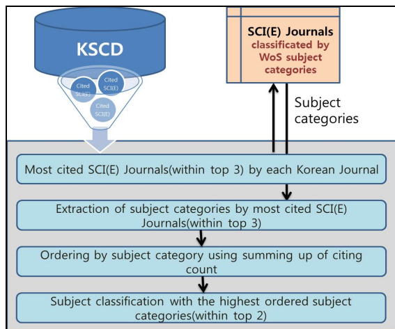
Fig. 3. Process of Automatic Subject Classification
