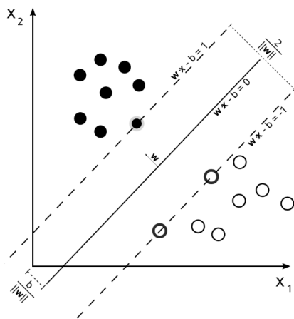
Fig. 2. Optimal maximum margin hyperplane of two classes. Samples on the margin correspond to support vectors
