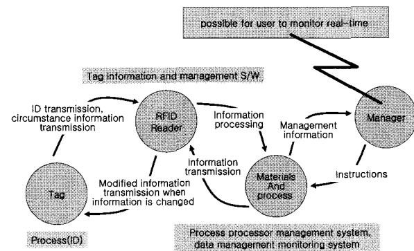
Fig. 2. System Structure
