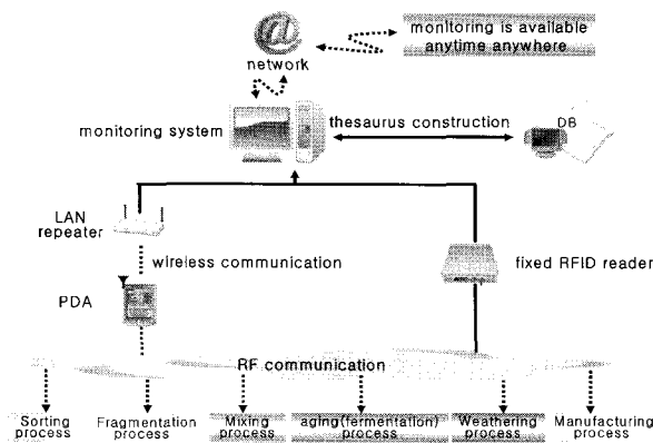
Fig. 1. The Structure of The Brick Manufacturing Process
