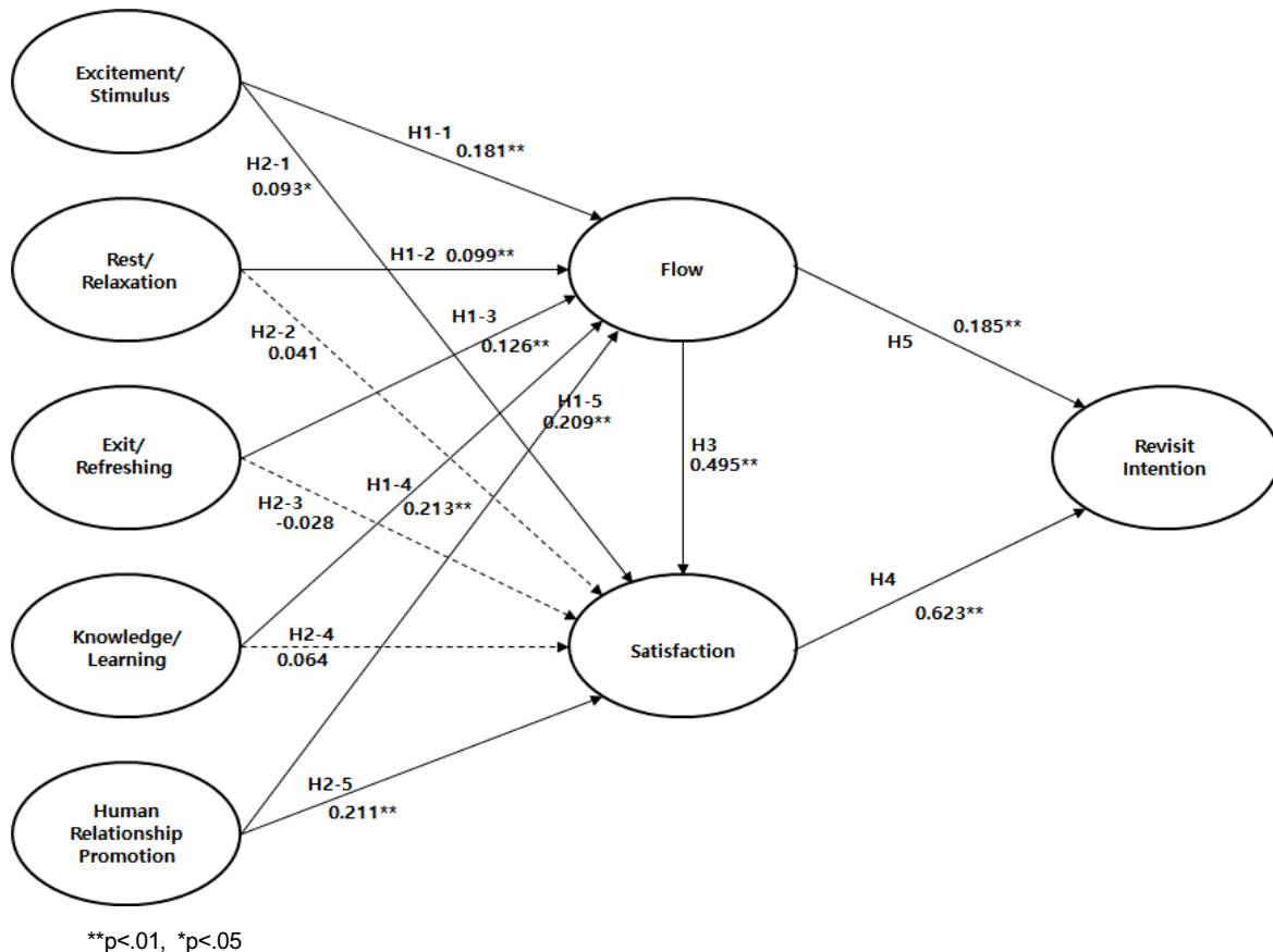
<Figure 1> Estimates of the structural model(PLS)
