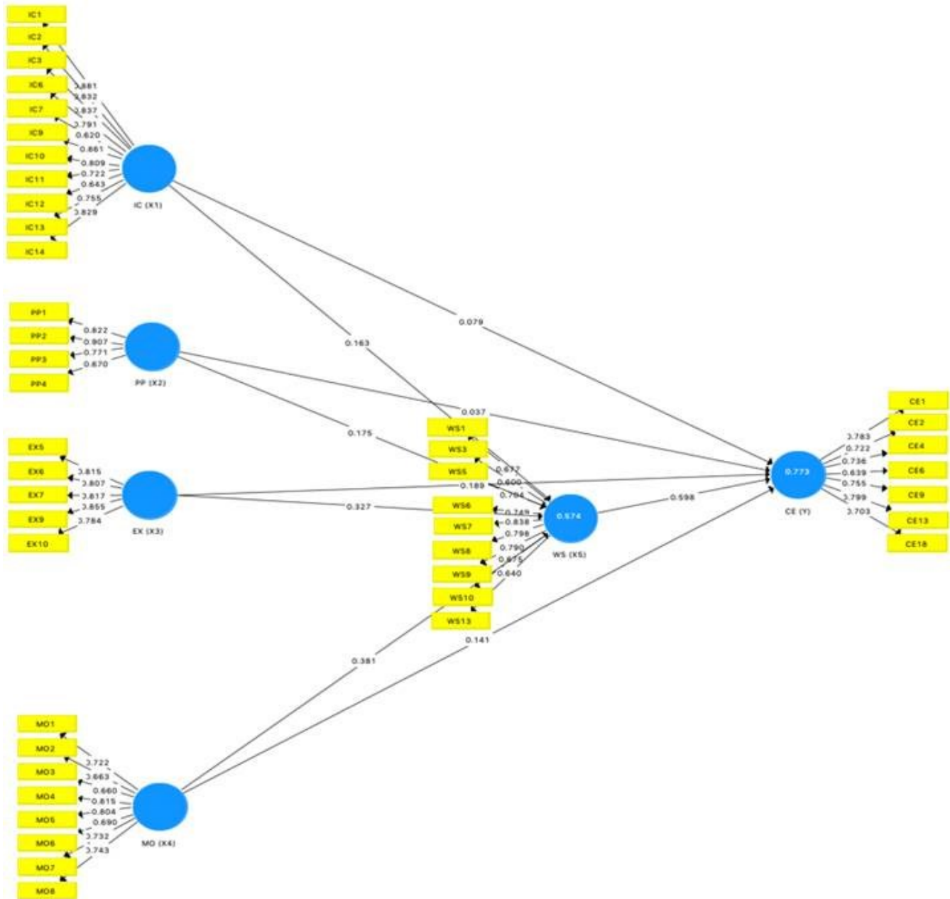
Figure 2: SmartPLS Model
