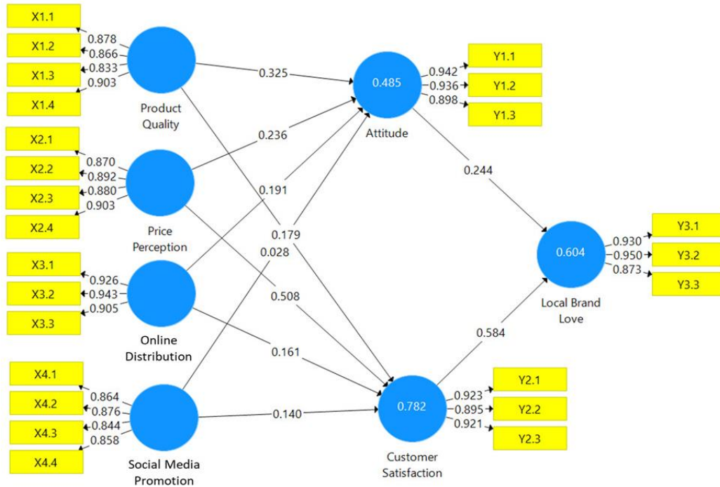
Figure 2. Structural Model
