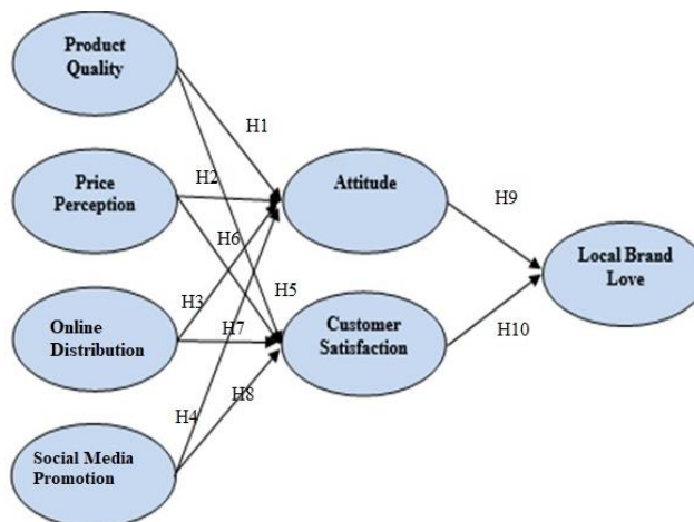
Figure 1: Conceptual Framework
