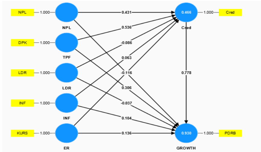
Figure 2 : Algorithm Analysis
