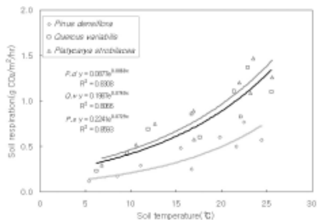
Fig. 4. The relationships between soil respiration rate and soil temperature for the three study sites.
