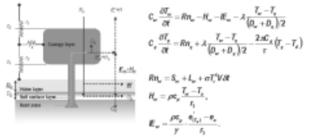
Fig. 3. Transfer pathways as conceptualized and parameterization in SiB2-Paddy.
