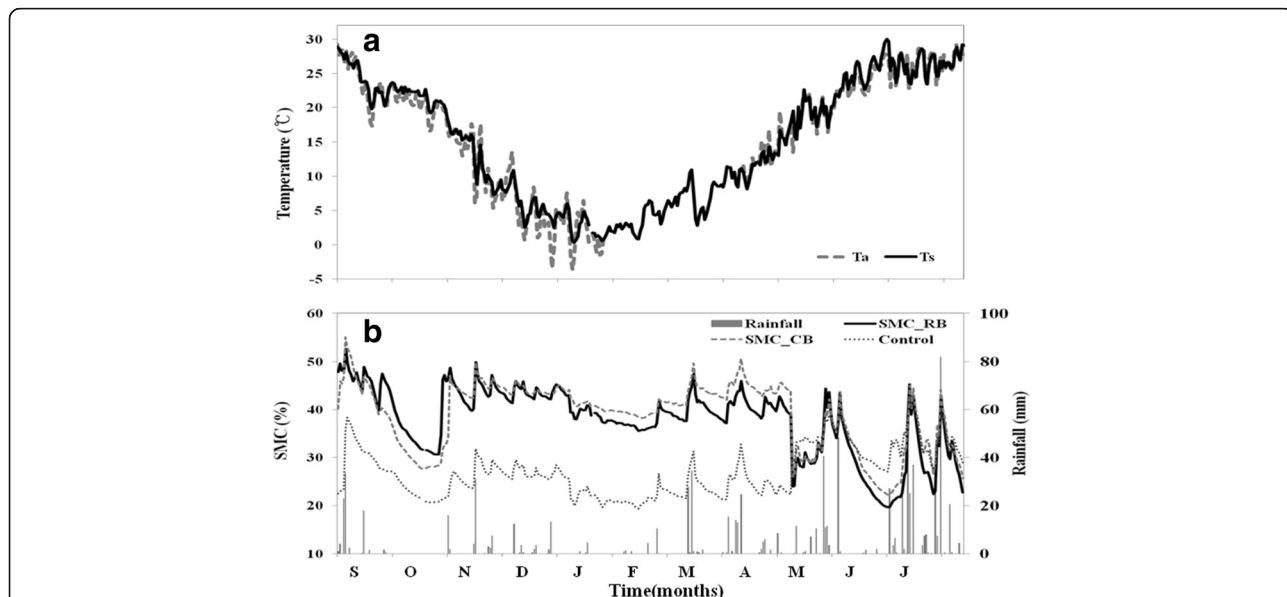
Fig. 2 Variation of soil temperature (Ts) at 5-cm depth, air temperature (Ta) (a), and soil moisture content in red pepper residue biomass section (SMC_RB), soil moisture content in carbonized biomass section (SMC_CB), soil moisture content in control section, and rainfall (b) in the first and second year at the experiment site
