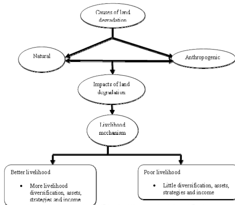
Fig. 1 Conceptual framework of land degradation-livelihood nexus
