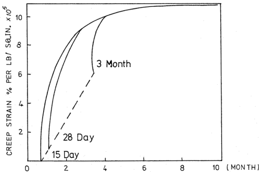
Fig. 9 variation in creep with age of concrete at loading
