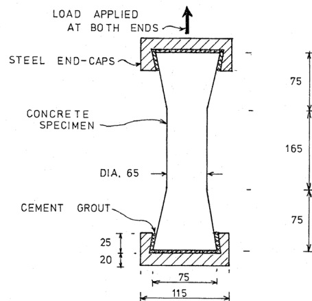
Fig. 13 Section through tensile specimen and end-caps.(Unit: mm)
