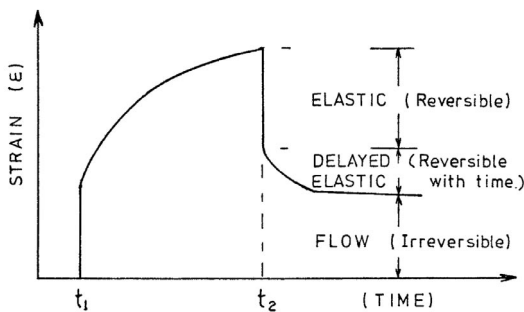
Fig. 5 Typical strain-time curve for concrete under sustained load
