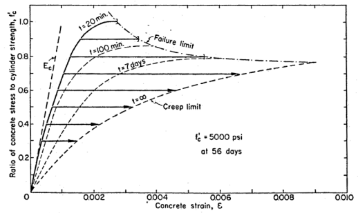
Fig. 12 Influence of load intensity and duration on concrete strain
