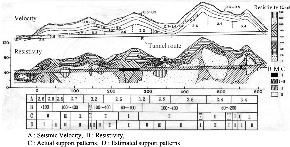
Fig. 6 Comparison of estimated support patterns with actual support patterns obtained from the railway tunnel in Japan
