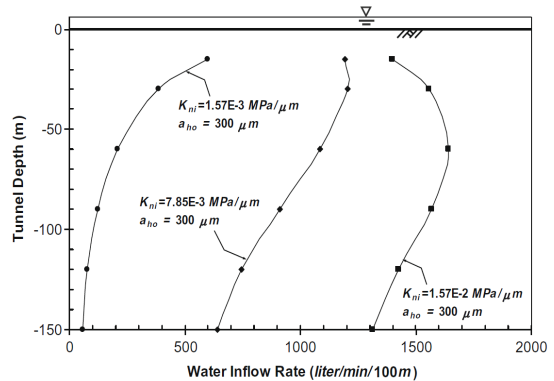
Fig. 11. Change of ground-water inflow rate with depth under various joint geological conditions
