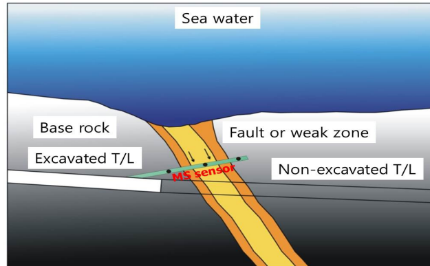
Fig. 8. Suggested MS monitoring plan for detecting the behavior of fault or weak zone during tunnel construction
