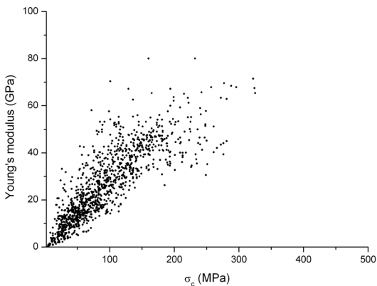
Fig. 4. Relationship between uniaxial compressive strength and young's modulus
