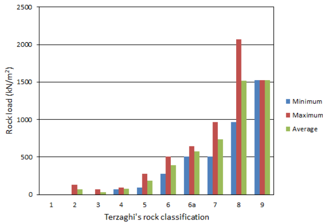
Fig. 4. Comparison of rock load by Terzaghi's rock load classification table (Park et al, 2013)
