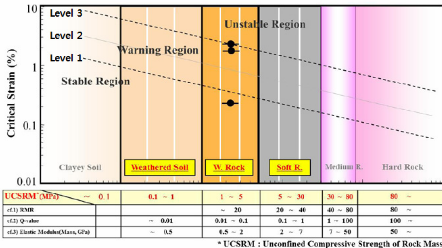
Fig. 14. A new critical strains diagram (Park, 2013)
