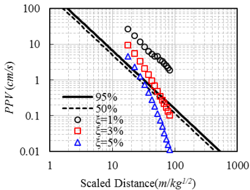
Fig. 6. Effect of damping on attenuation curve (duration =0.001s)
