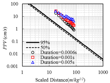
Fig. 5. Effect of duration of the blast load on the attenuation relationship
