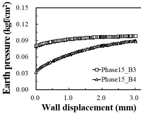
Fig. 19. Pressure on B3 and B4
