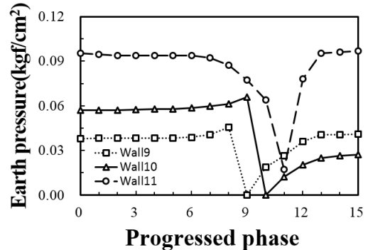
Fig. 36. Pressure for bulging, W9,10 & B1
