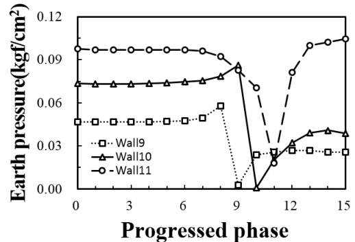
Fig. 35. Pressure for cantilever, W9,10 & B1
