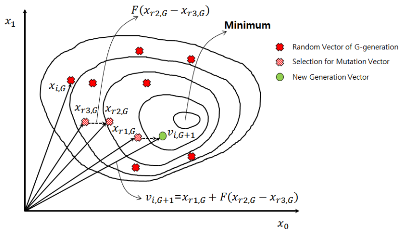
Fig. 5. DEAP process in two-dimensional space (Storn and Price, 1997)
