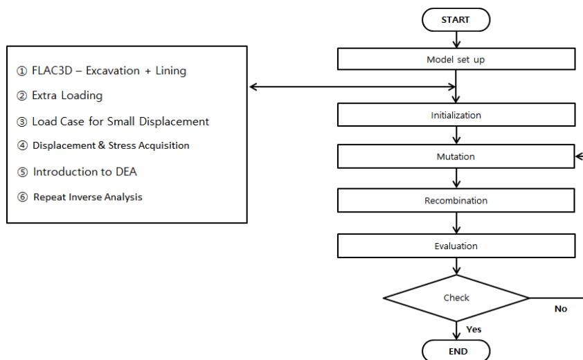
Fig. 2. Flowcharts of back analysis for initial input parameters (displacements and stresses) (An et al., 2016)
