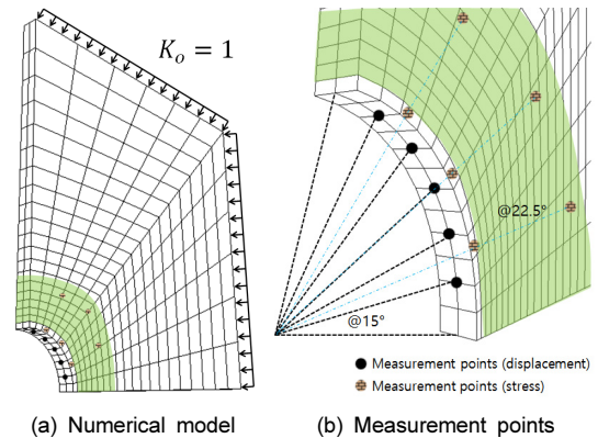
Fig. 5. Numerical model and measurement points for the feasibility study of displacement-stress-stiffness degradation based DEA
