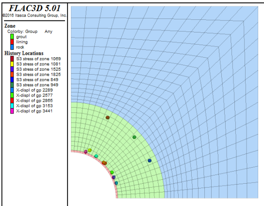
Fig. 7. FLAC3D Numerical Model and measurement points of displacement-stress-stiffness degradation based DEA
