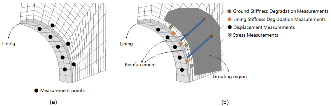
Fig. 3. The comparison of previous and current feasibility study for measurement points of DEA (a) displacement-stress based points (b) displacement-stress-stiffness degradation based points
