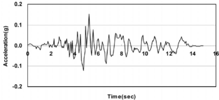
Fig. 4. Acceleration time history of the Hachinohe wave
