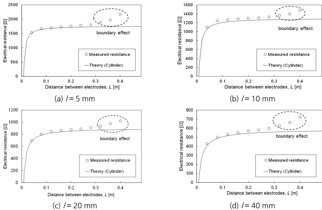
Fig. 4. Theoretical & experimental resistance and boundary effects ( \rho = 29.97 \Omega\text{m} )
