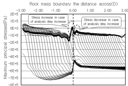
(c) Maximum principal stresses at crown in case of 4&5
