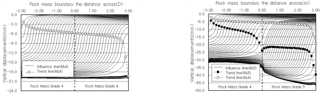
(a) Influence line and trend line in case of 4&4
