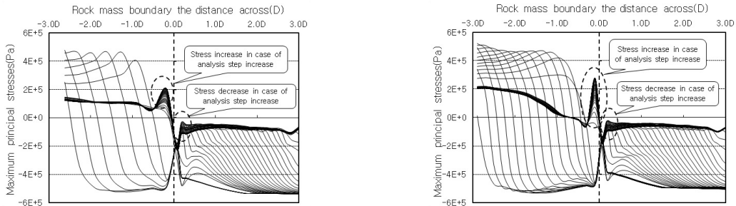
(a) Maximum principal stresses at crown in case of 2&5
