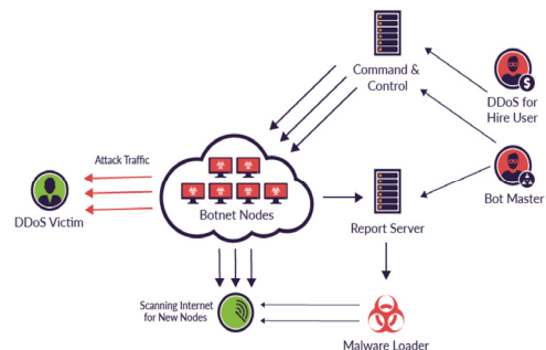
[Fig. 4] IoT Botnet Malware Flow diagram
