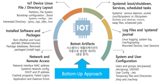
[Fig. 6] Target for collecting artifacts on IoT devices
