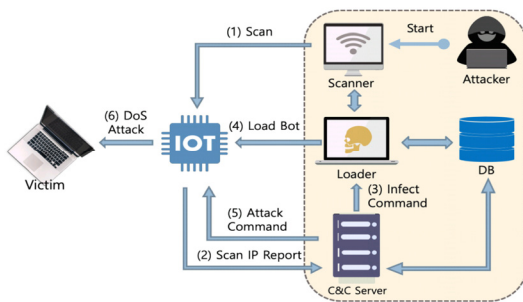
[Fig. 3] IoT Bot infection procedure diagram
