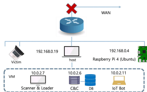
[Fig. 2] Network diagram to replay IoT Botnet
