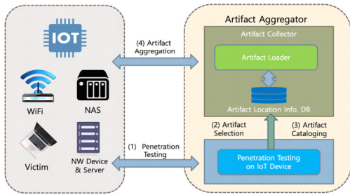
[Fig. 5] Structure diagram of an intrusion artifact collector for IoT devices
