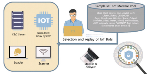
[Fig. 1] Select IoT Botnet to be analyzed and replay its behavior
