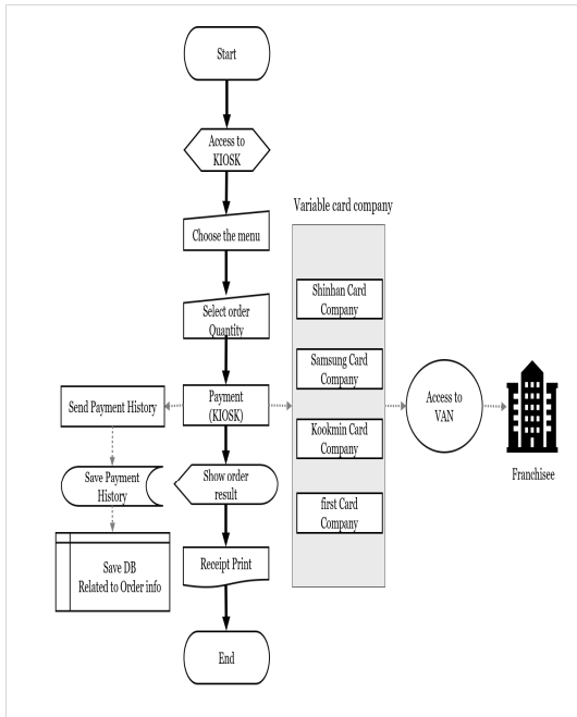
[Fig. 1] Kiosk Payment System [10]
