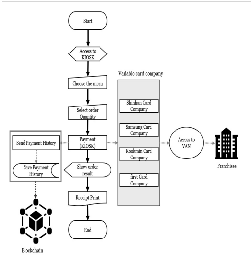
[Fig. 3] A System Proposal Full Protocol
