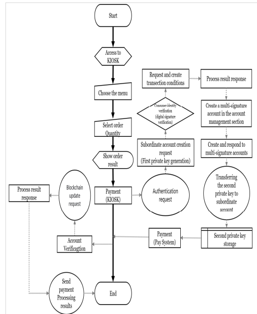
[Fig. 2] The mechanism of "credit virtual currency generation device and credit virtual currency management device" released by ShinhanCard[11]
